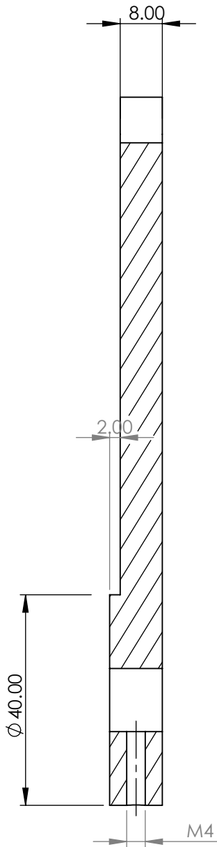
SECTION B-B
